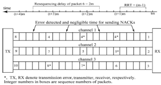
Fig. 2. MSW-ARQ-inS ( M = 3 , m = 5 ).
