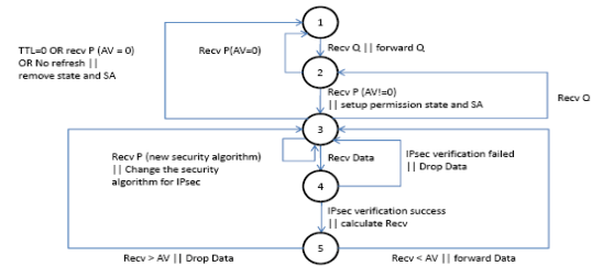
c) Router (State 1: Idle, 2: Wait for P, 3: Permission state, 4: IPsec verification, 5: Compare RV and AV)
