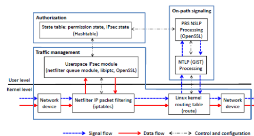
Fig 4: PBS Implementation
