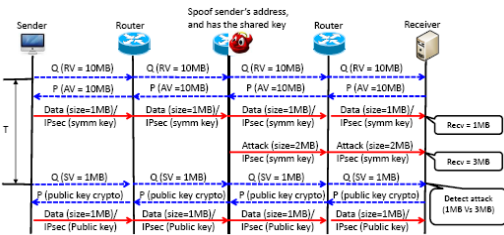
Fig. 2. Basic operation of the PBS Detection Algorithm (SV: The volume of data that the sender has sent; Recv: The volume of data that the receiver has received; size: data size) system.
