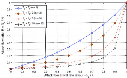
Fig 3: Attack Flow Ratio
