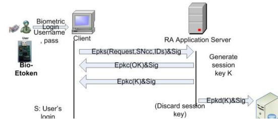
Fig.4. Sequence diagram for Remote Access Control
